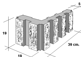
plaqueta L
